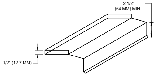
SILL PAN FLASHING DETAIL
