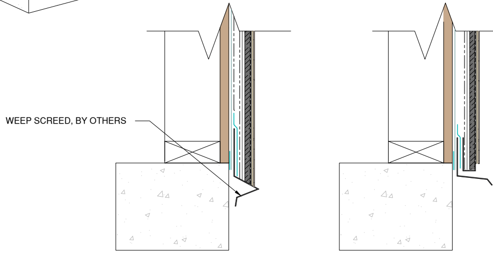
WEEP SCREED OPTION SECTION DETAIL
