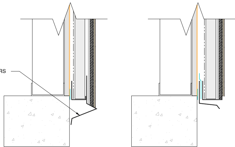
WEEP SCREED OPTION SECTION DETAIL
