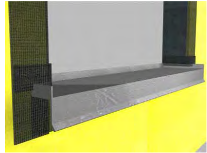
Apply AquaFlash System over vertical flashing legs.
